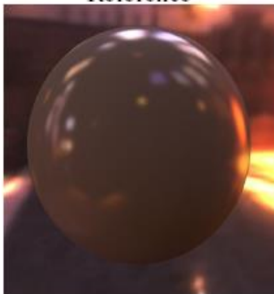
Lafortune: 0.0486
