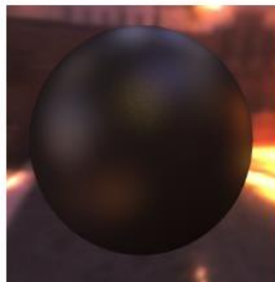
Ward: 0.0137
