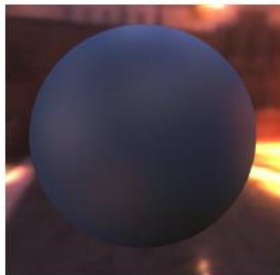
Ward: 0.00956
