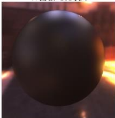
CT: 0.00307
